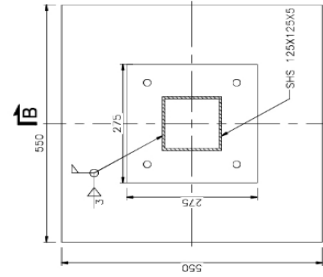
CONCRETE BLOCK DETAIL
